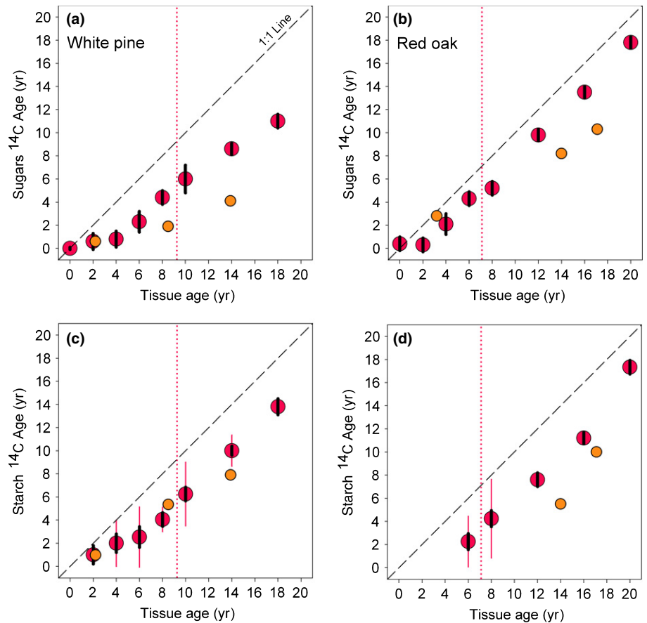
Fig. 3 Radial trends in radiocarbon ( 14 C) age (see the Materials and Methods section) of extracted sugars (a, b) and starch (c, d) in stemwood and large coarse root samples of white pine ( Pinus strobus , a, c) and red oak ( Quercus rubra , b, d). For stemwood, tissue age was determined by direct ring counts. For roots, tissue age was determined by 14 C analysis of extracted cellulose (see the Materials and Methods section). The vertical dotted line indicates the sapwood–heartwood boundary at breast height. The thin red vertical error bars indicate the standard deviation of 14 C age across repeat samples (where available; see Supporting Information Methods S1). The heavier black vertical bars indicate the analytical uncertainty (one standard deviation, 1 SD) of the accelerator mass spectrometry (AMS) measurements (see Methods S1).
